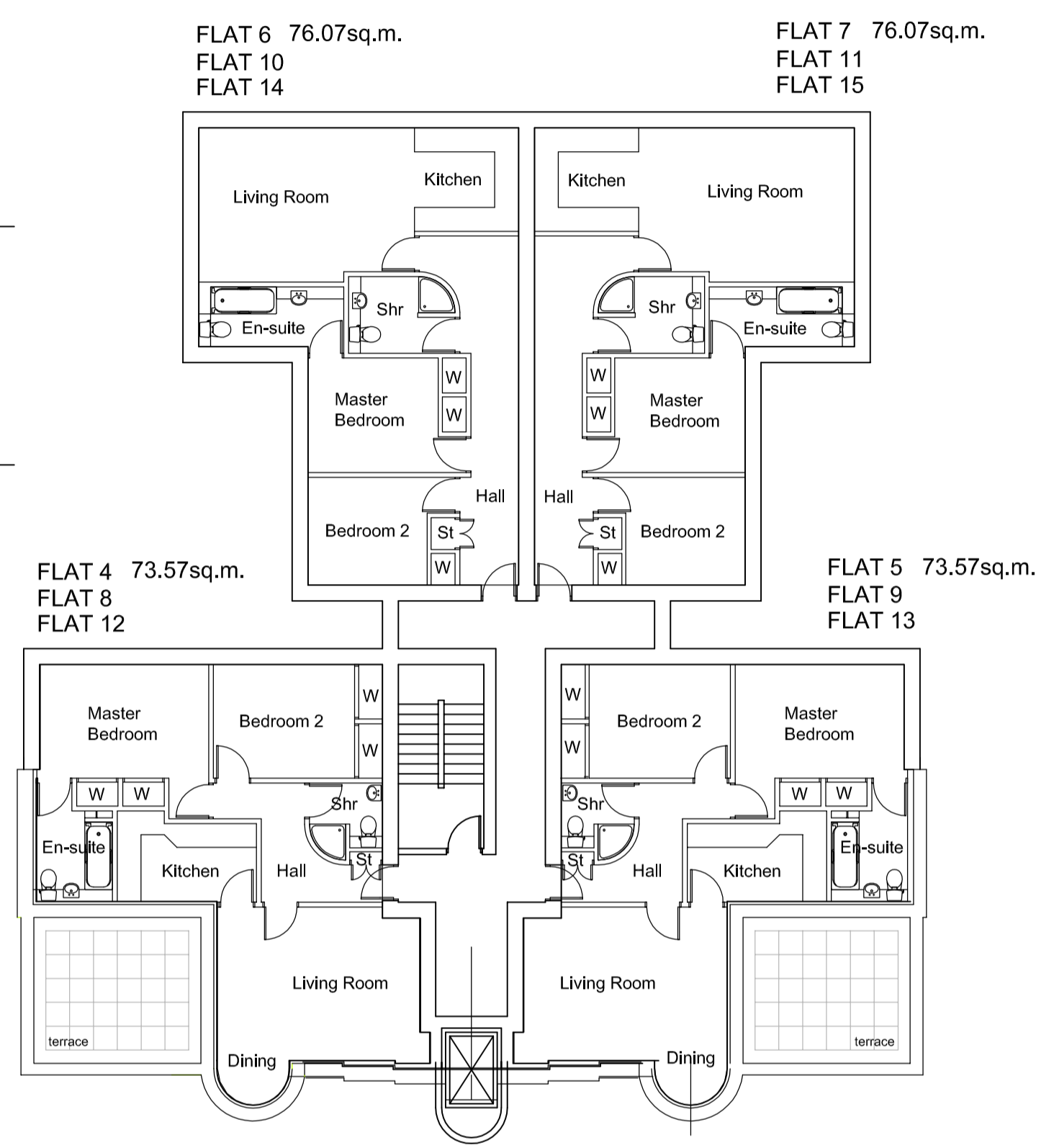
FIRST TO THIRD FLOOR PLAN [AS PROPOSED]
