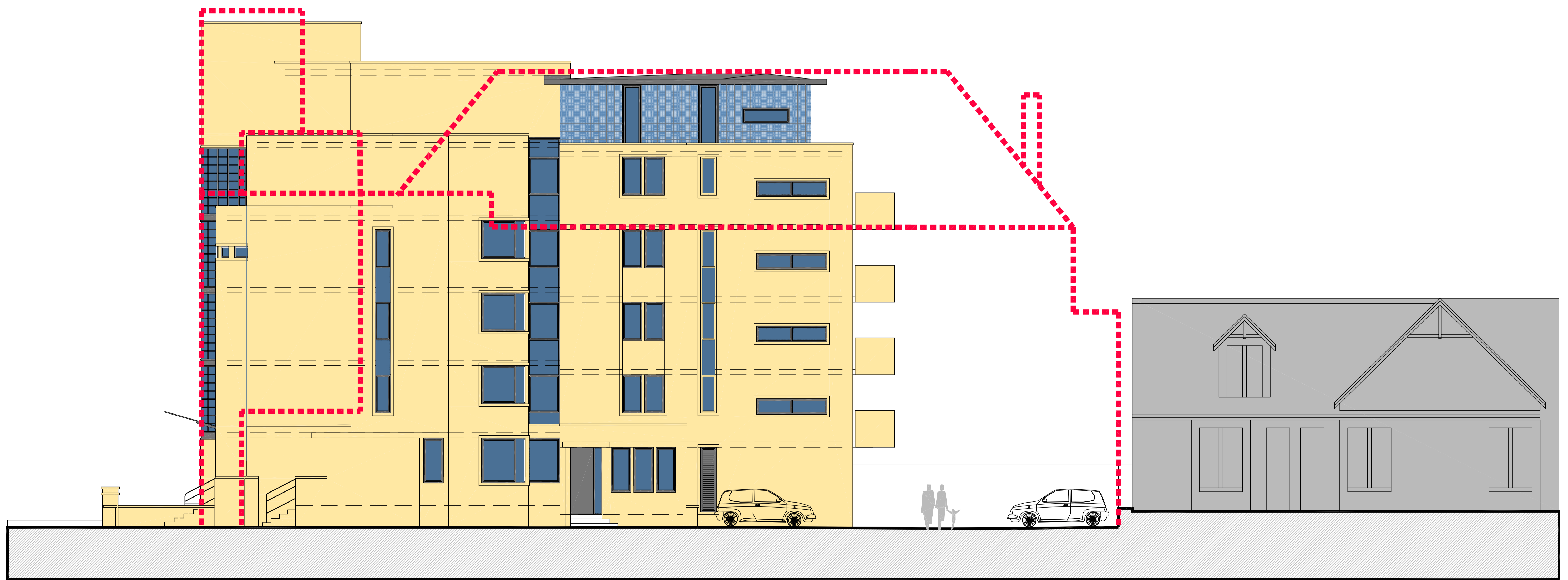
EAST ELEVATION [AS PROPOSED WITH ORIGINAL BUILDING OVERLAYED]
