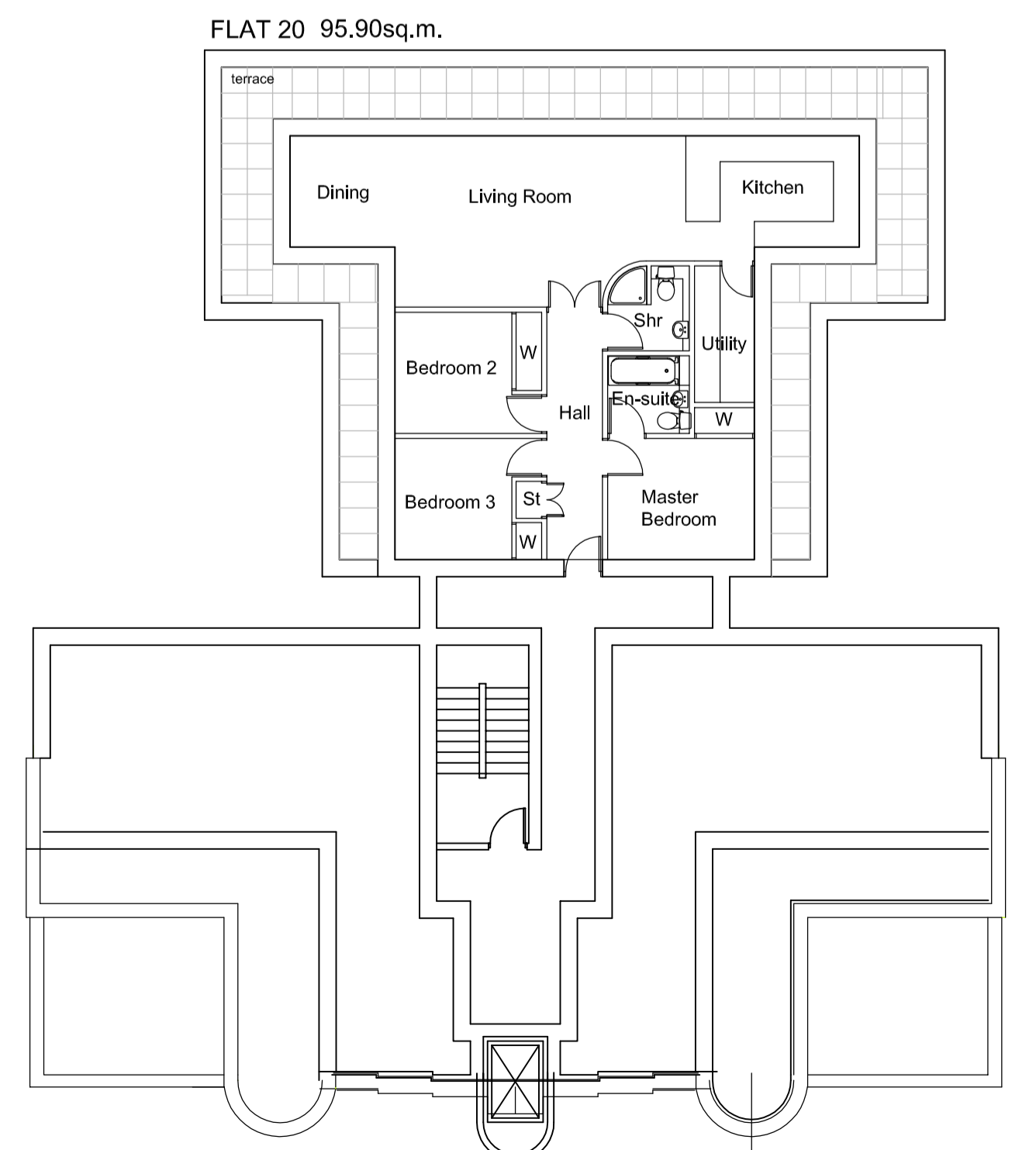
FIFTH FLOOR PLAN [AS PROPOSED]
