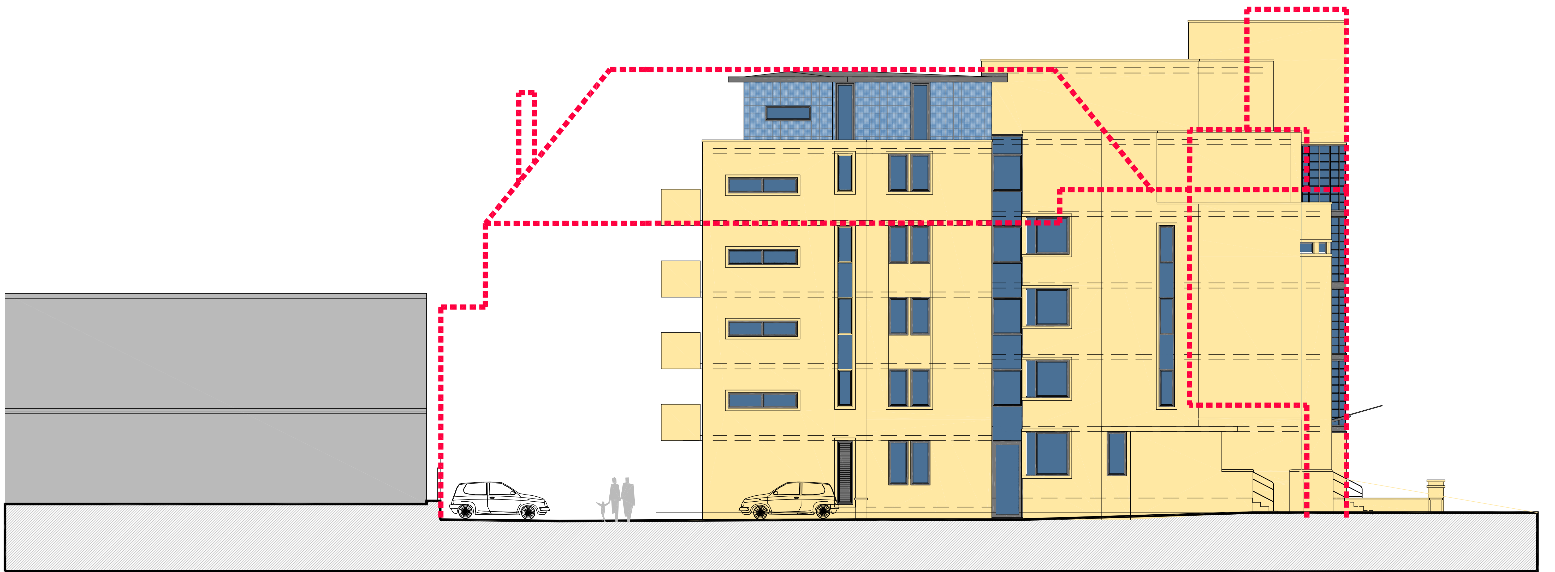
WEST ELEVATION [AS PROPOSED WITH ORIGINAL BUILDING OVERLAYED]
