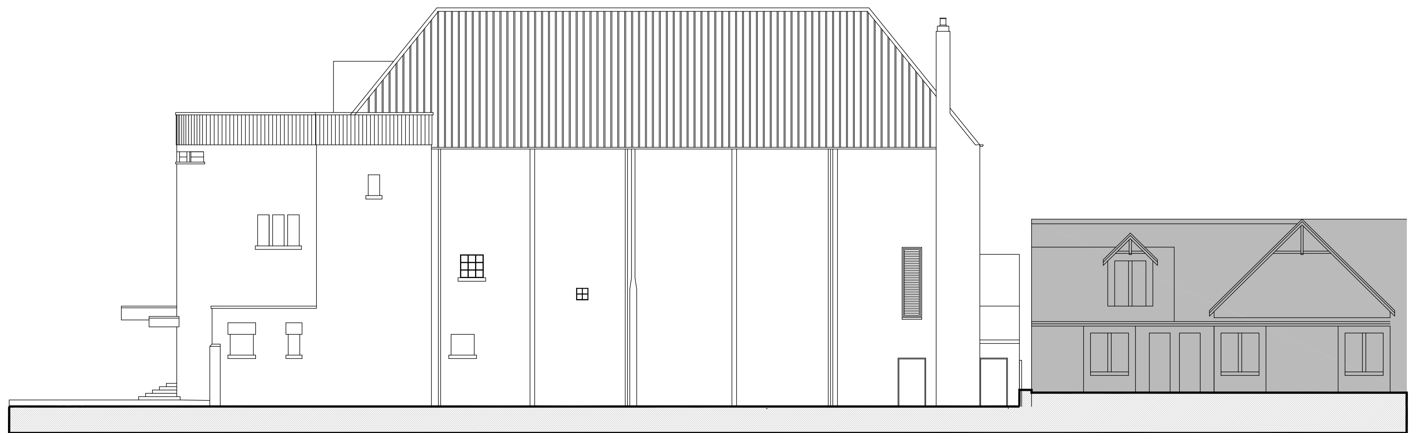
EAST ELEVATION [AS EXISTING]
