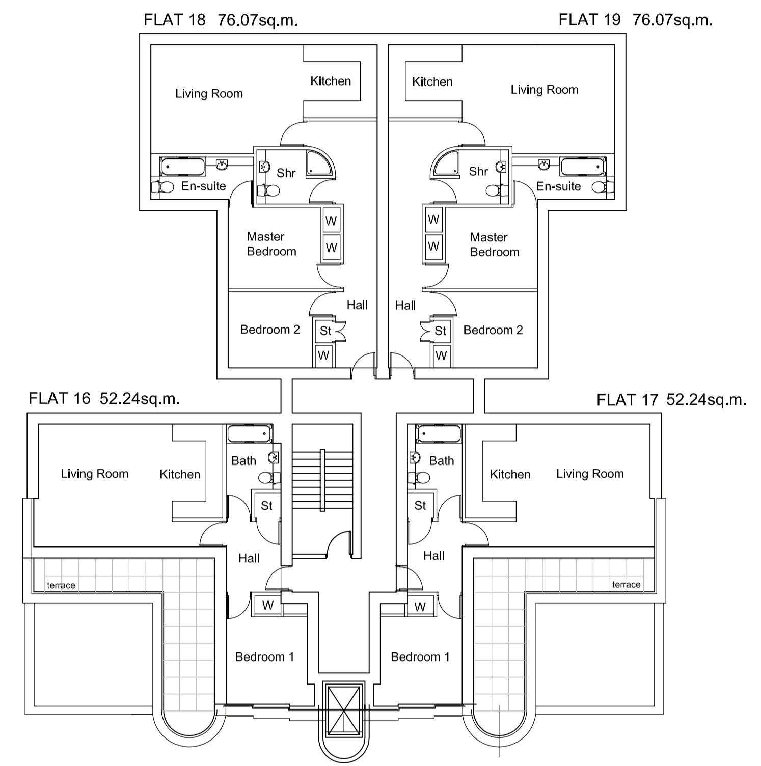
FIFTH FLOOR PLAN [AS PROPOSED]
